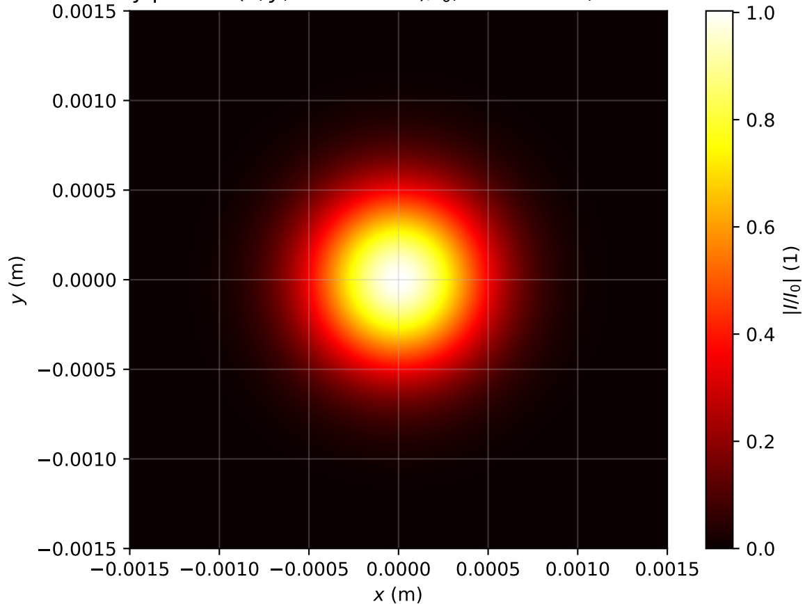
Intensity profile I(x, y, z = 0.080m)/I_0 , P_{in}=0.7P_{cr} , artificial time
